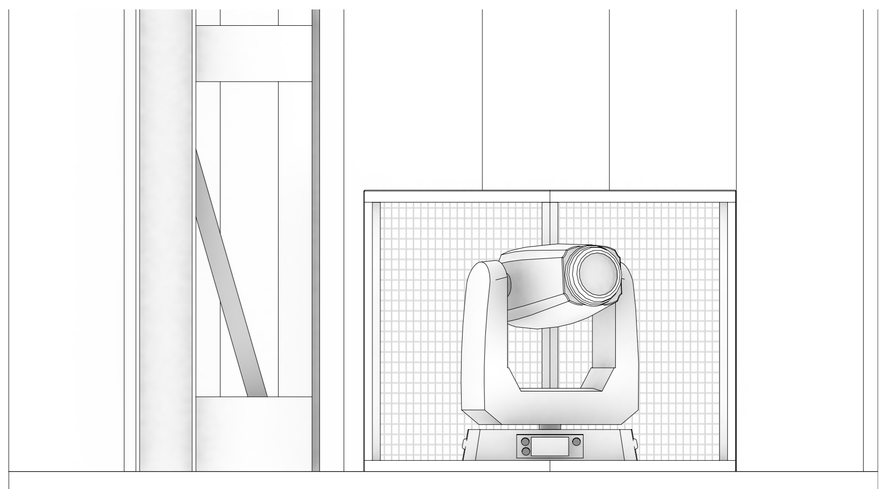
3 MOVING LIGHT CRATE (CAGE ROOM 2) Scale: 1:10
