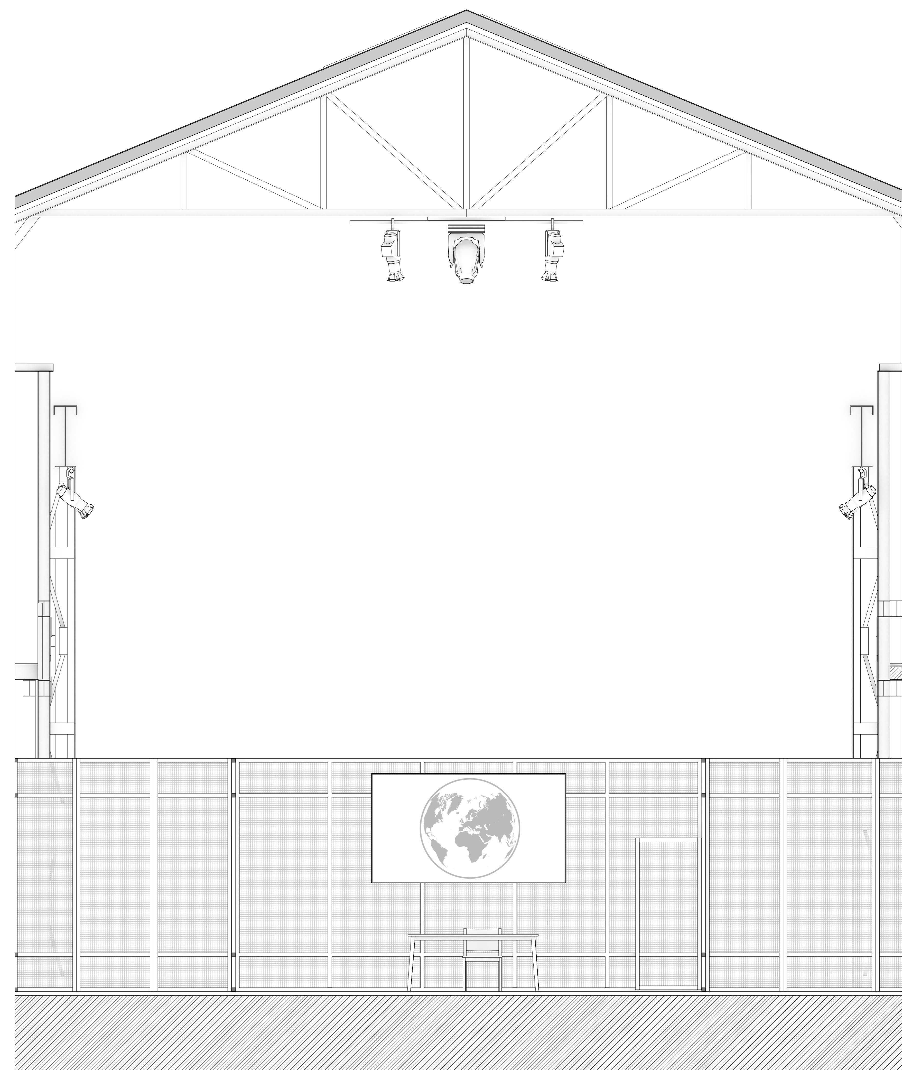
3 NORTH FACING Scale: 1:25
