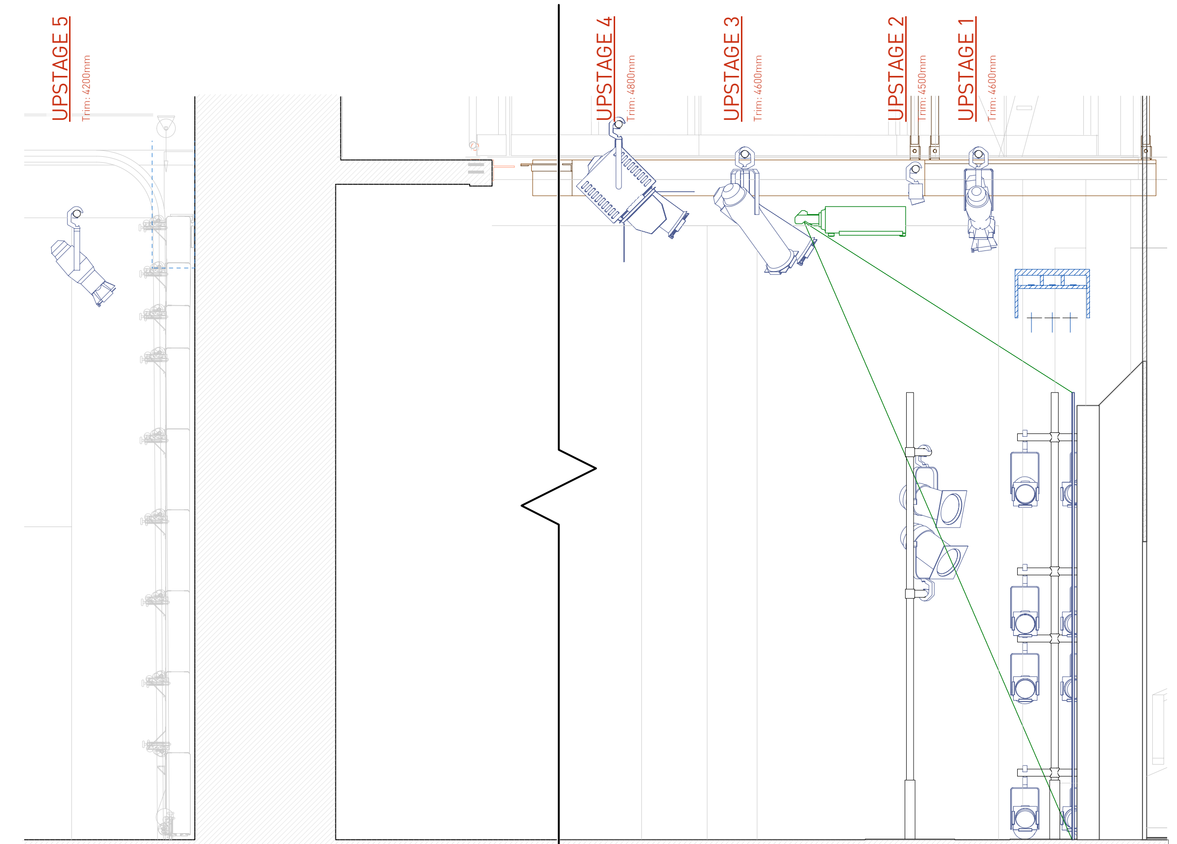
1 LIGHTING UPSTAGE 5 Scale: 1:25
